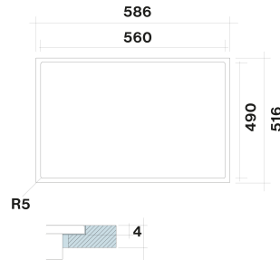
Flush installation
